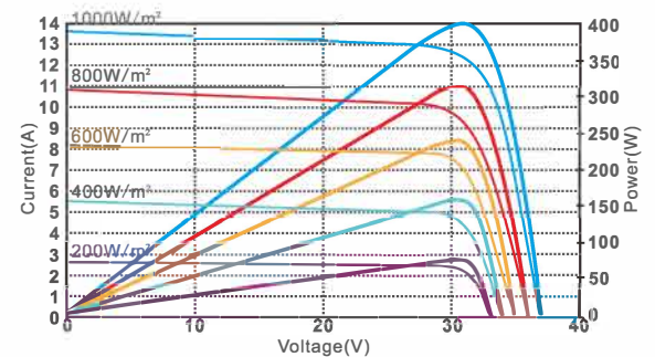
I-V characteristics at different irradiancies
