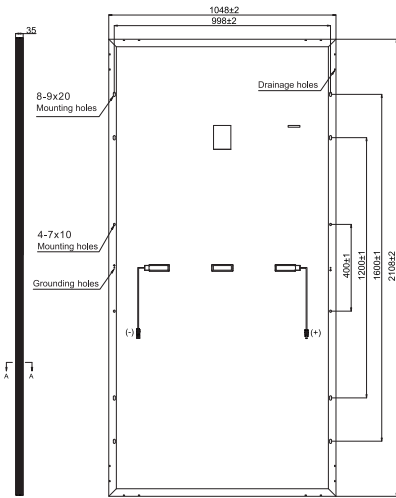
Dimensions of PV Module Unit: mm
